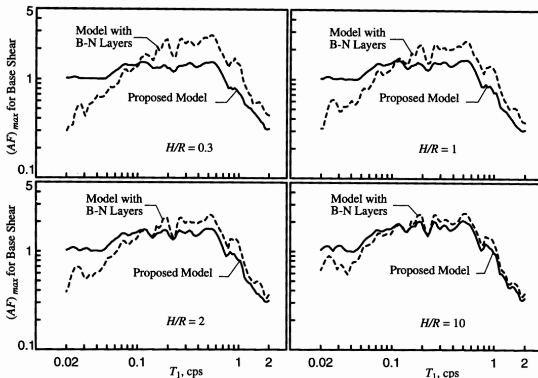
Fig. 22 Maximum amplification factor for amplitude of base shear induced by El Centro record; \nu = 0.3 , \delta = 0.1
