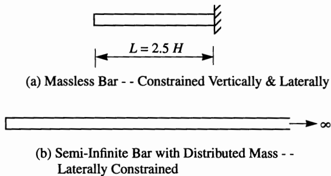
Fig. 15 Representation of soil-stratum in Scott's model and its variant.
