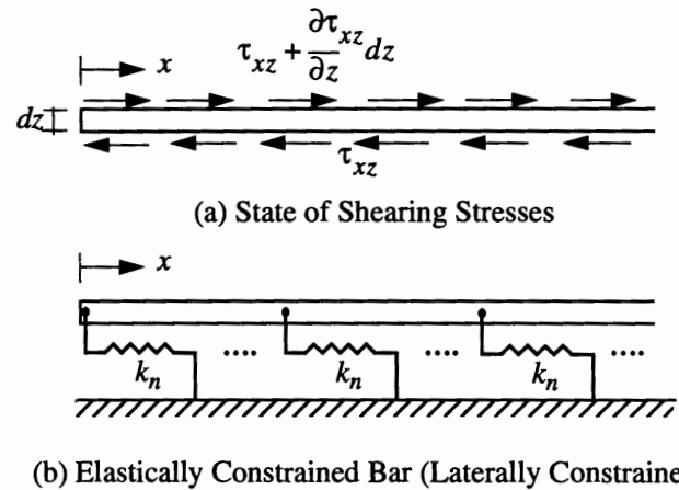
Fig. 16 Exact modeling of soil-stratum
