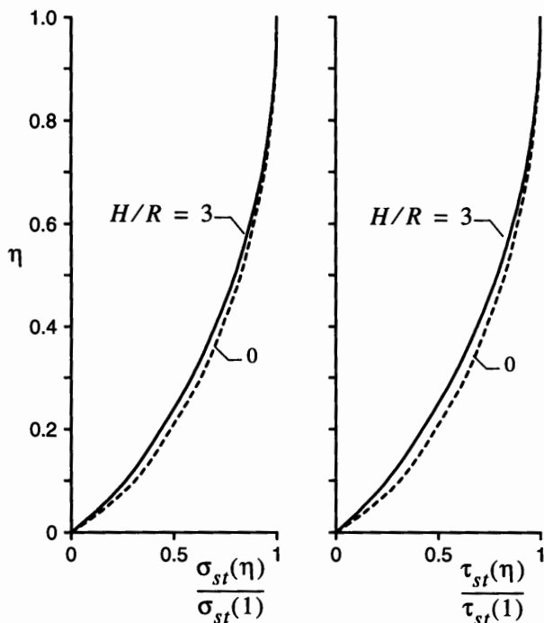
Fig. 3 Heightwise variations of static values of normal and circumferential wall stresses; rough interface, \nu = 0.3 .
