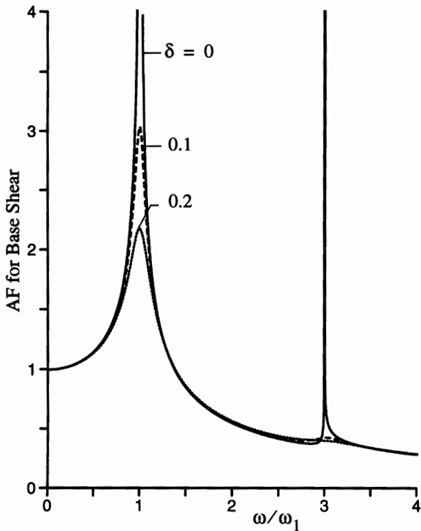
Fig. 9 Effect of material damping on frequency response curves for base shear in straight walls; \nu = 0.3 .
