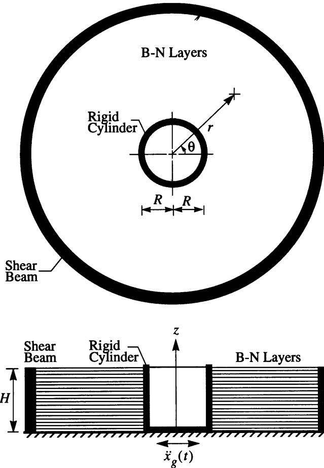
Fig. 18 Model for system with embedded cylinder
