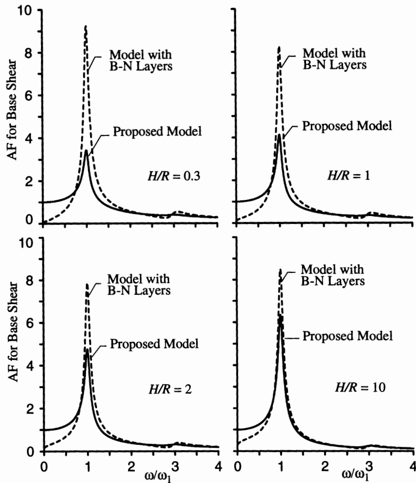
Fig. 21 Frequency response curves for amplitude of base shear in harmonically excited systems; \nu = 0.3 , \delta = 0.1
