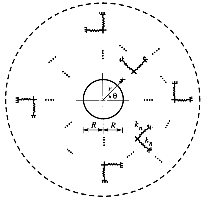
Fig. 19 Elastically constrained thin layer
