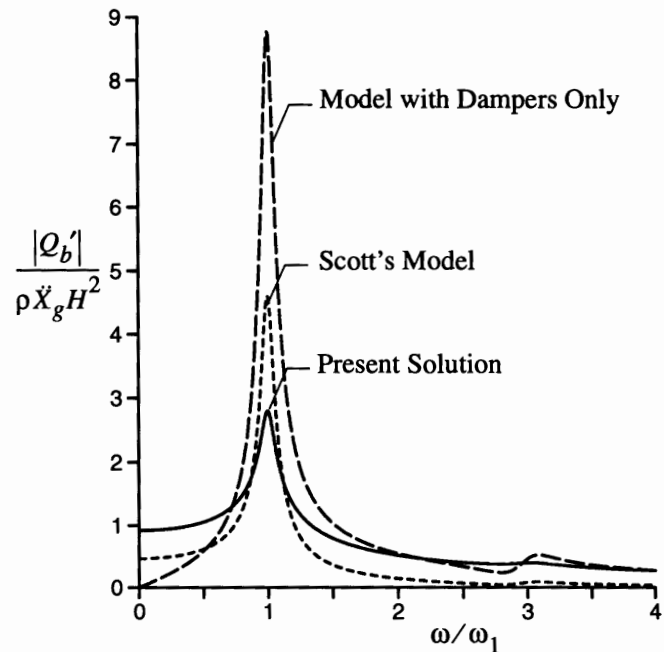
Fig. 14 Frequency response curves for base shear amplitude in straight walls; \nu = 0.3 & \delta = 0.1 .
