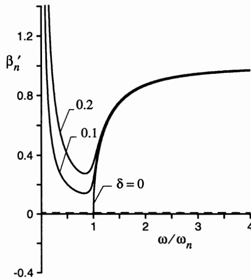
Fig. 17 Stiffness and damping factors for elastically constrained bar; straight wall.
