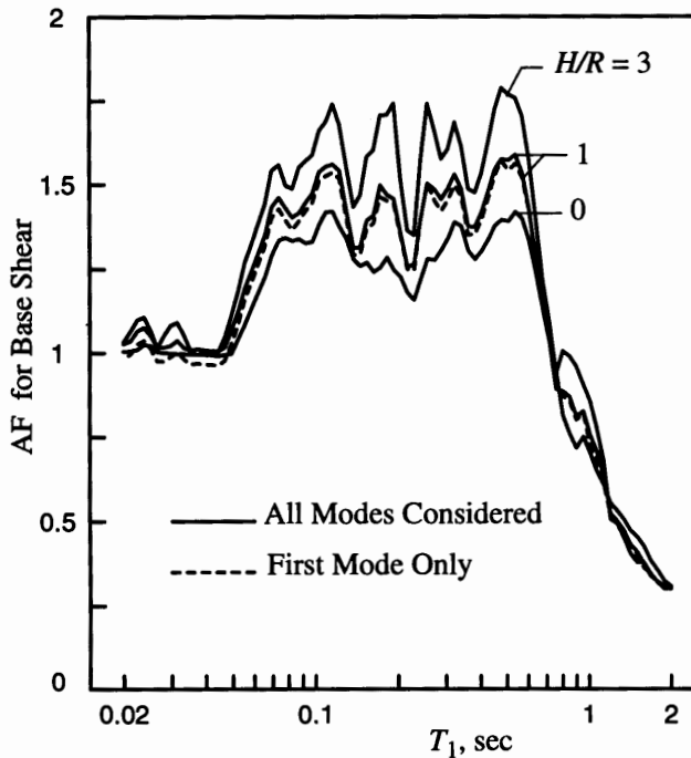
Fig. 11 Amplification factors for base shear due to El Centro record; rough interface, \nu = 0.3 & \delta = 0.1 .
