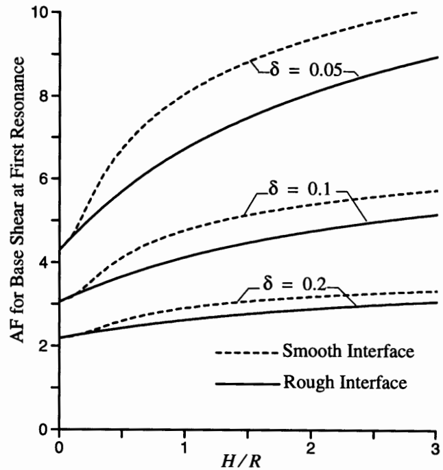
Fig. 10 Effect of slenderness ratio & material damping on resonant amplification factor for base shear; \nu = 0.3 .
