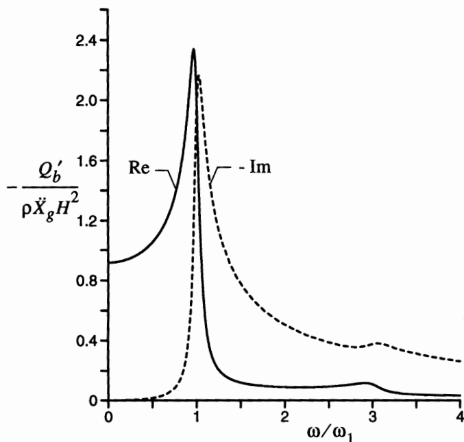
Fig. 7 Frequency response curves for base shear in straight walls; \nu = 0.3 & \delta = 0.1 .
