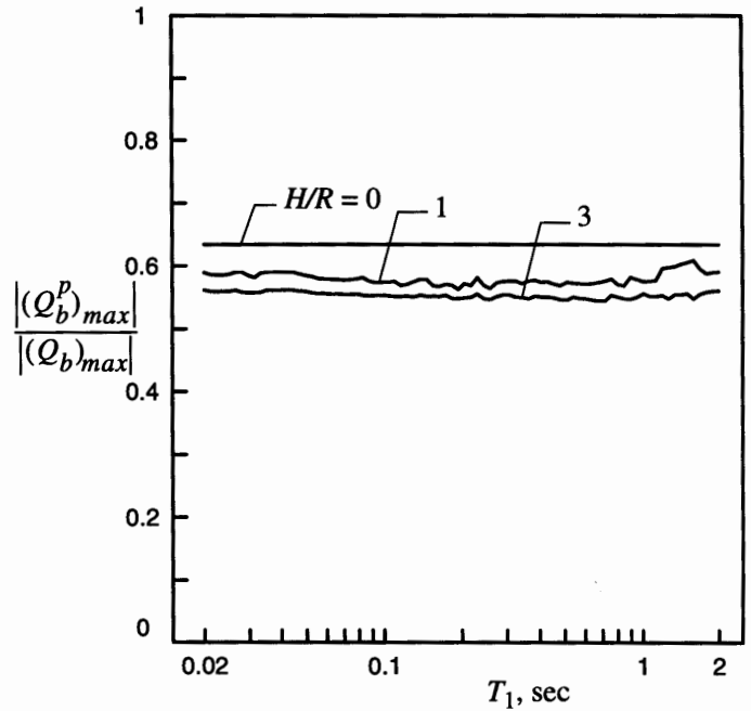
Fig. 12 Portion of maximum base shear contributed by pressures; rough interface, \nu = 0.3 & \delta = 0.1 .
