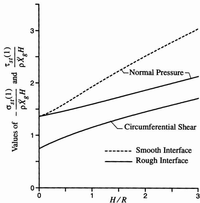
Fig. 4 Maximum values of normal and circumferential stresses; \nu = 0.3 .
