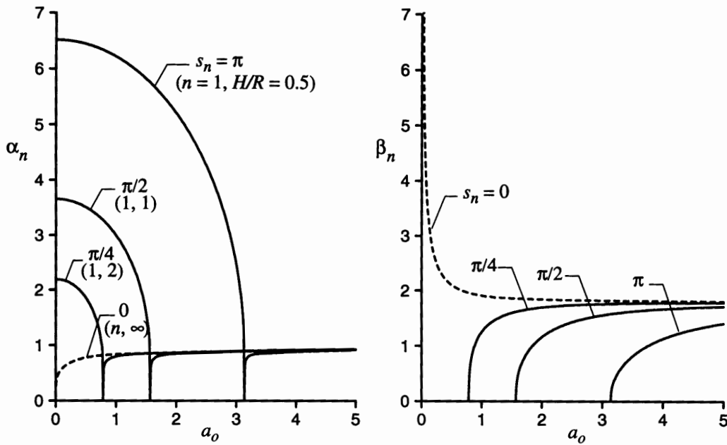
Fig. 20 Stiffness and damping factors for elastically constrained thin layer; \nu = 0.3 , \delta = 0 .
