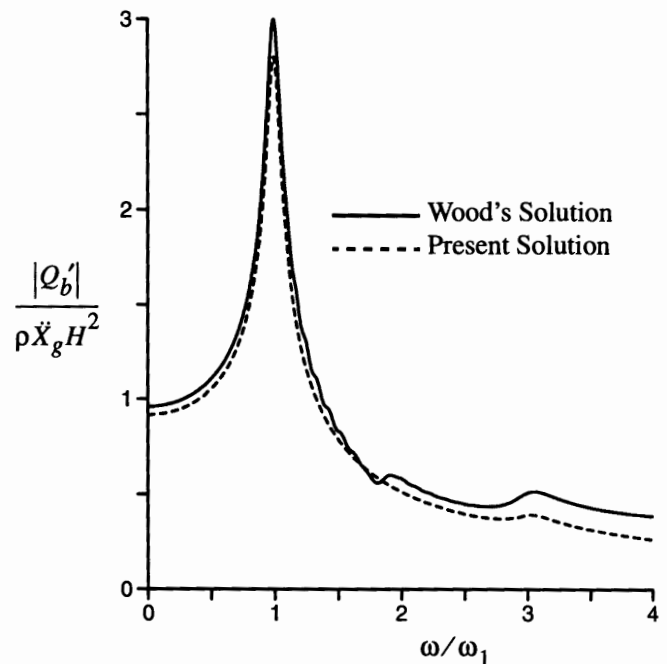
Fig. 8 Frequency response curves for base shear amplitude in straight walls; \nu = 0.3 & \delta = 0.1 .
