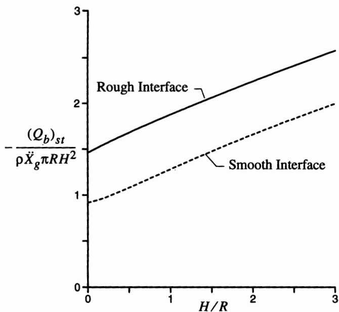
Fig. 5 Static values of total force or base shear for cylinder; \nu = 0.3 .
